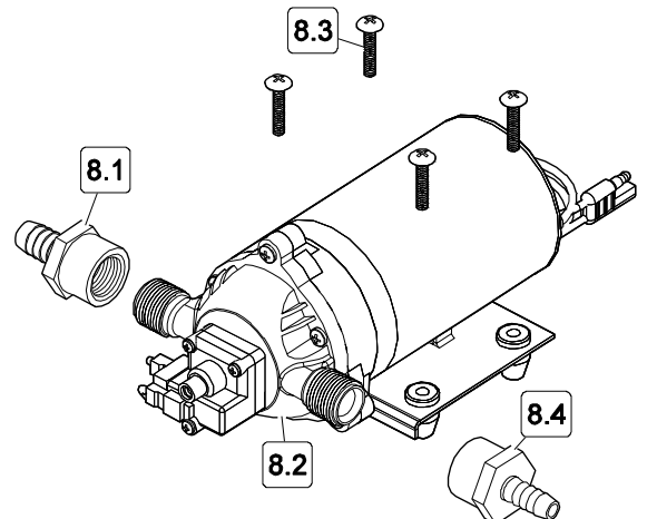
Pump Assembly Detail
